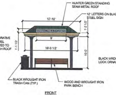
6 REST STOP SHELTER SCALE: NTS
