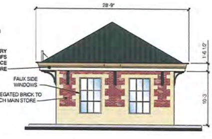
4 LEFT SIDE ELEVATION SCALE: NTS
