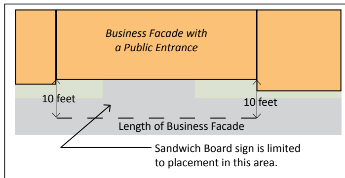
FIGURE 6.17(A): PERMITTED SANDWICH BOARD LOCATION
